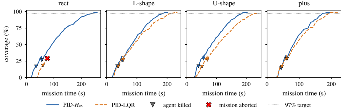
FIGURE 6. Coverage against mission time (coordinator clock). Triangles: agent kills, after which the failed cell is re-swept; dotted: 97% reference level (completion is defined by the survivors finishing their lanes).
